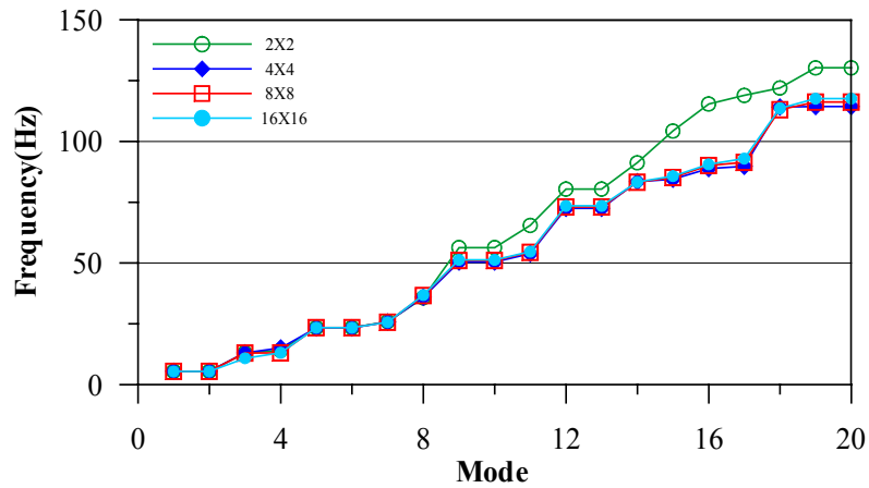
Fig. 3 Comparison of natural frequencies of a floor with different mesh division
