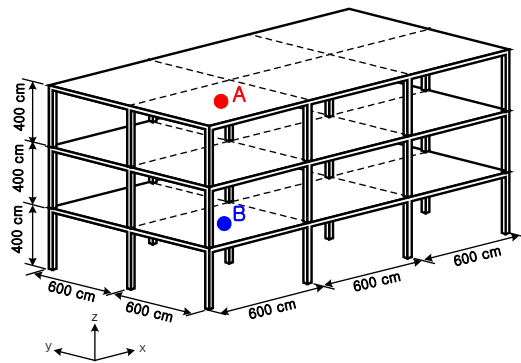
Fig. 12 Example structure with slabs
