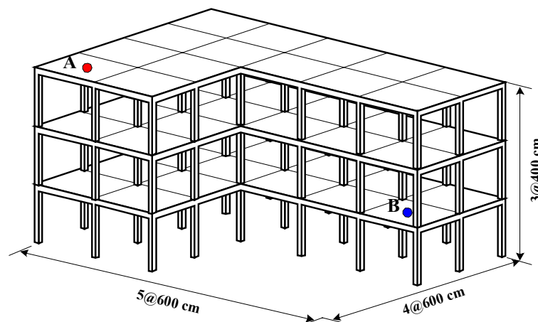
Fig. 18 Analytical model for unsymmetric building structure
