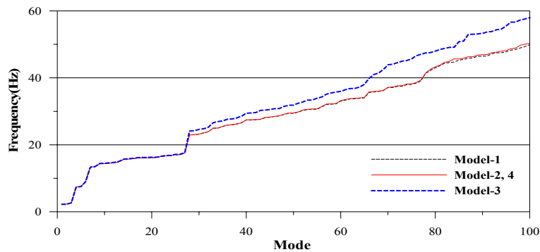
Fig. 15 Comparison of the natural frequency
