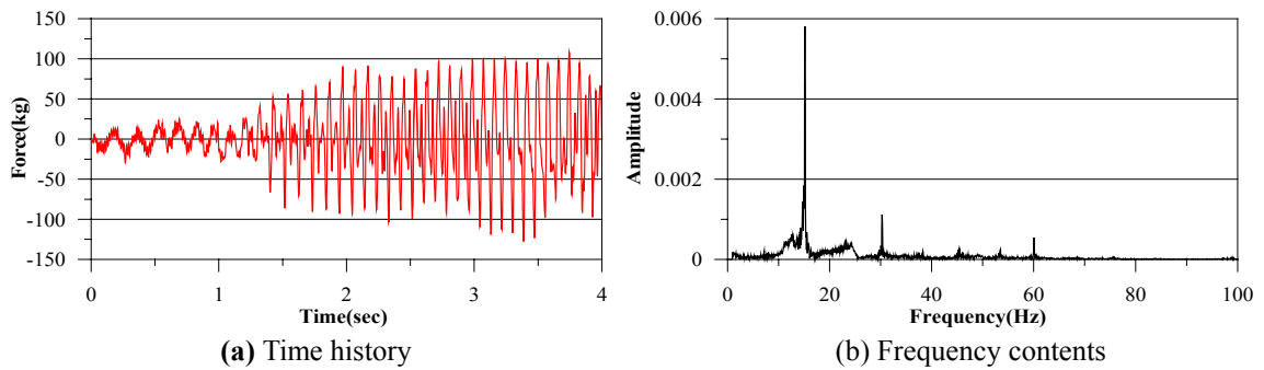
Fig. 13 Dynamic load applied at point A
