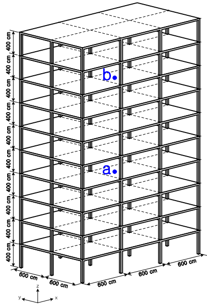
Fig. 21 Analytical model for large building structure 1
