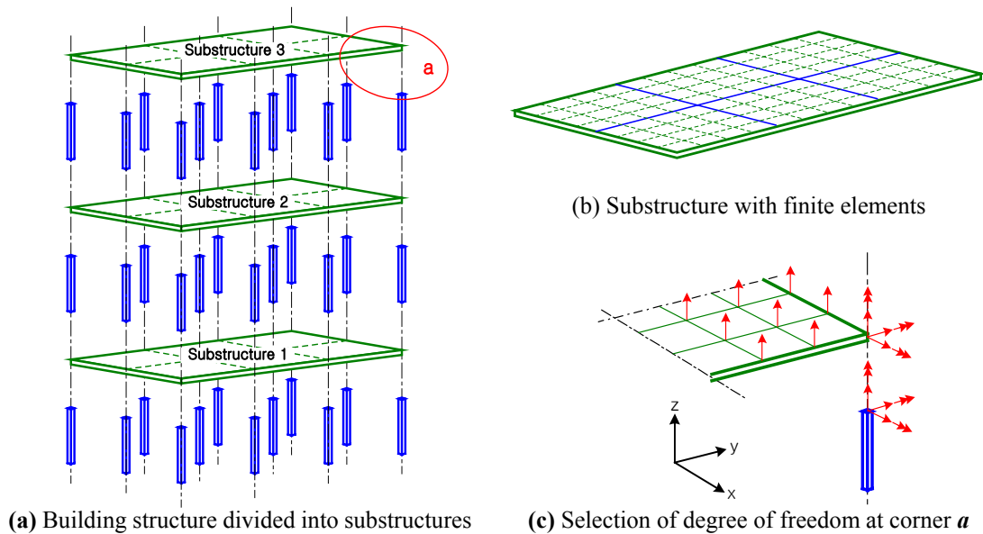
Fig. 9 Selection of substructure and master degrees of freedom
