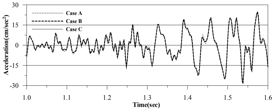
Fig. 19 Acceleration responses at node A
