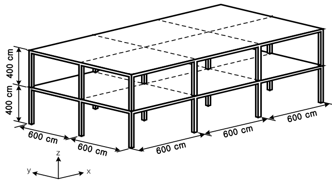
Fig. 4 Example structure with many slabs
