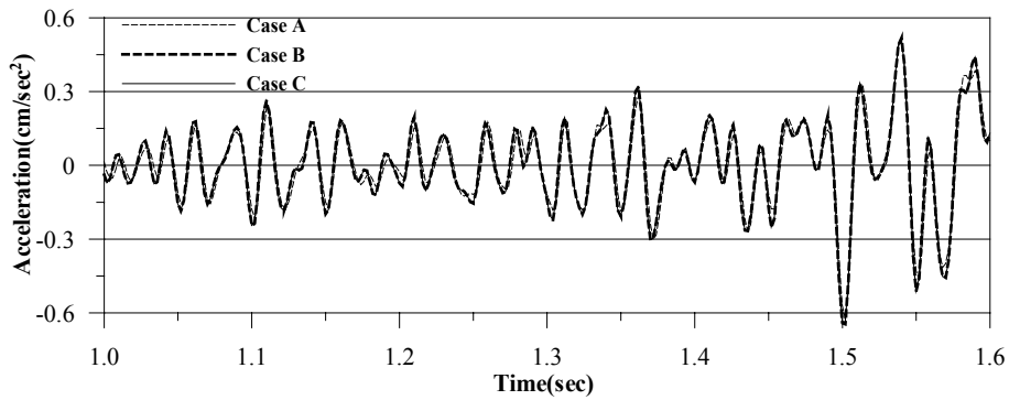
Fig. 20 Acceleration responses at node B
