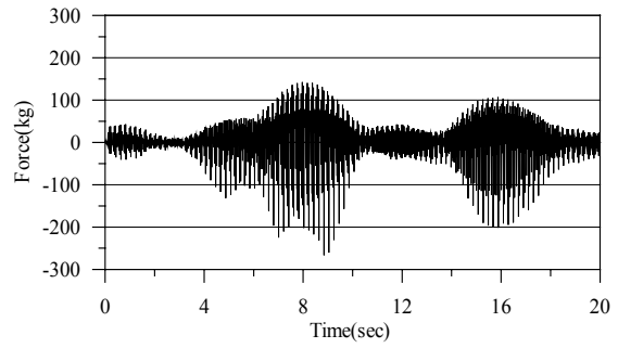
Fig. 22 Dynamic load Applied at point a
