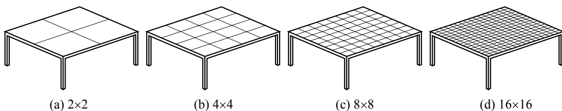
Fig. 2 Mesh division of a slab for floor vibration analysis
