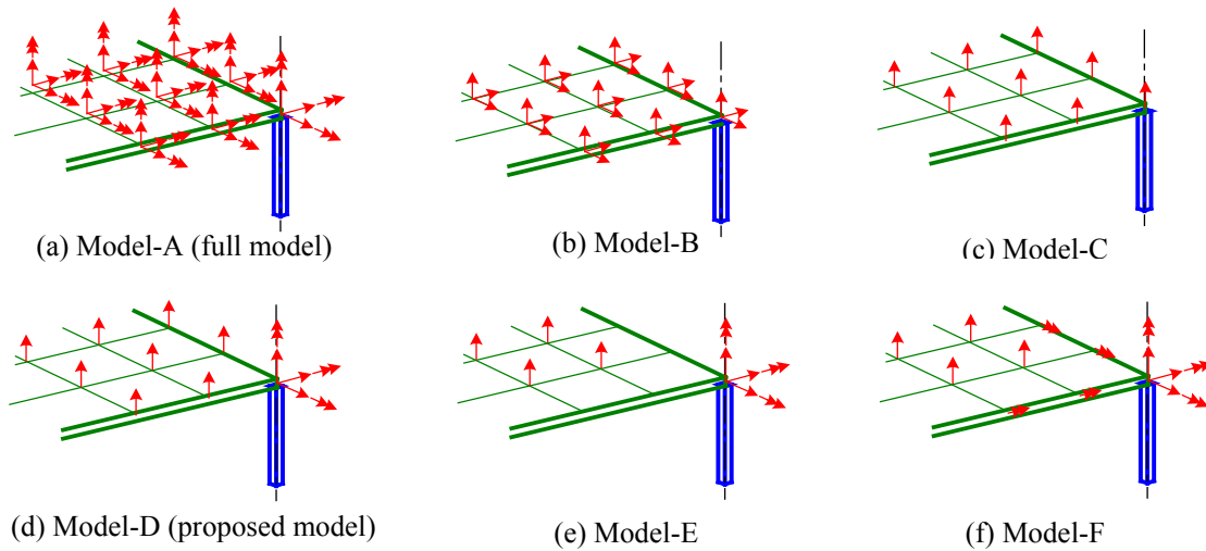
Fig. 8 Selected master DOF's for various selection criteria
