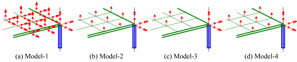
Fig. 14 Selected master DOF's for the example structure
