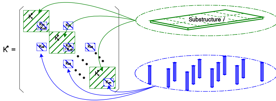
Fig. 11 Construction of stiffness matrix for global system
