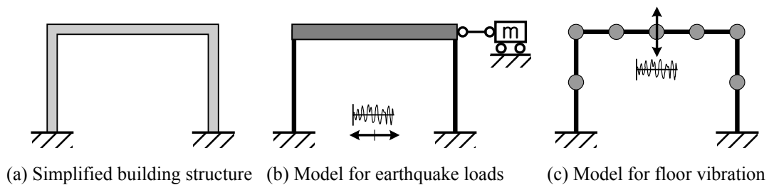
Fig. 1 Analytical modeling of a building structure
