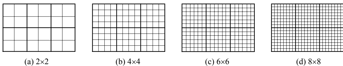
Fig. 5 Mesh division for floor vibration analysis
