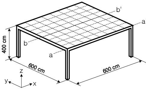
Fig. 6 8x8 finite element division of slab
